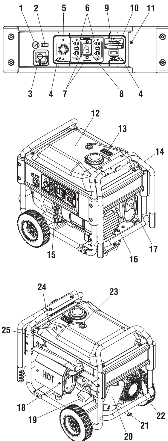
Figure 3 – Generator Locations
