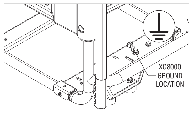
Figure 6 – Generator Ground Location
