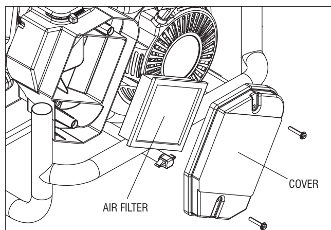
Figure 13 – Air Filter
