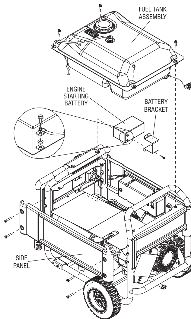
Figure 16 – Battery Removal
