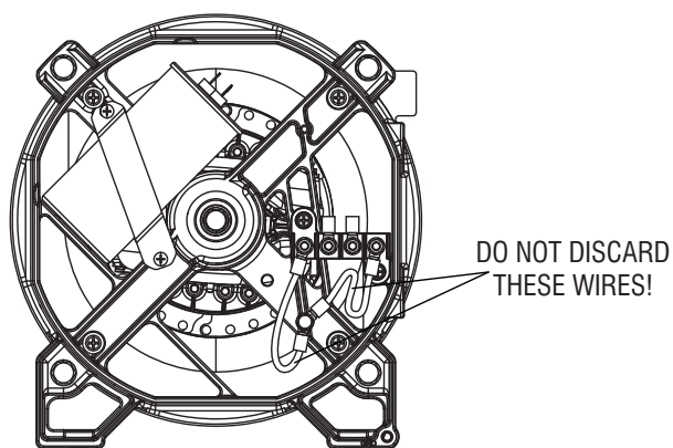
Figure 7 – Neutral to Frame Ground
