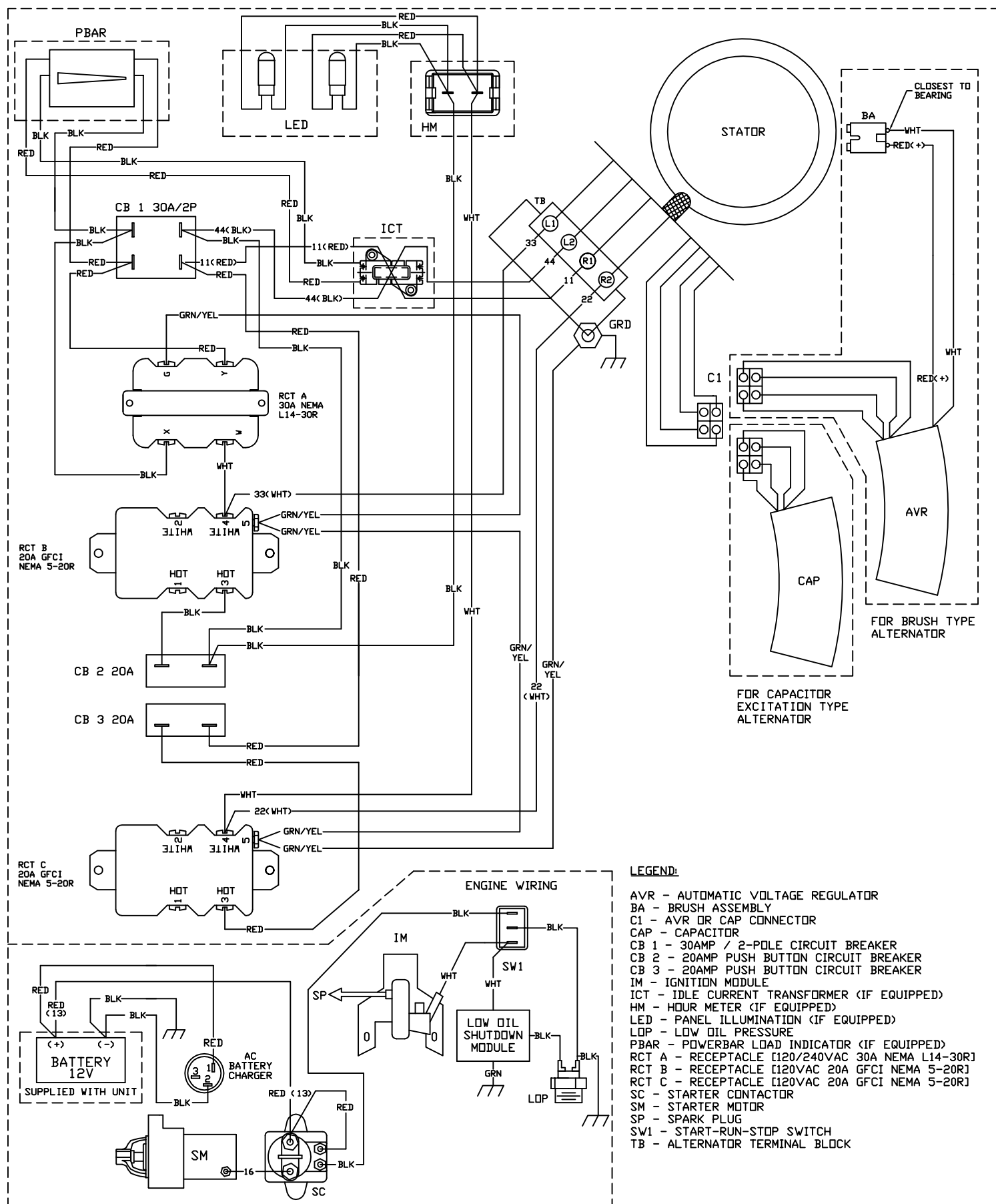
WIRING - DIAGRAM XG8000 CAL/CSA DRAWING #: 0H5277
